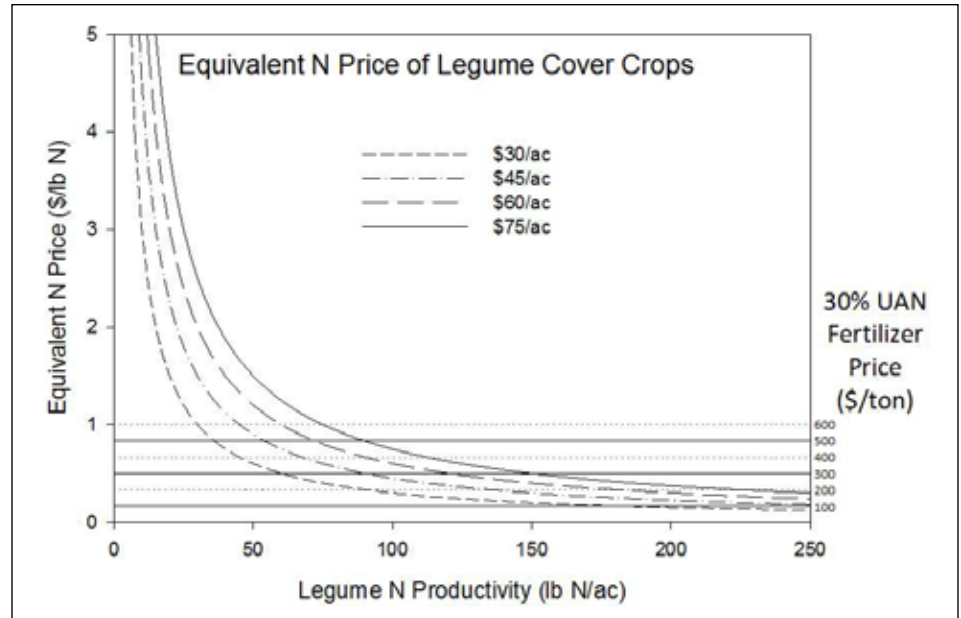
Figure 9. Equivalent N price of specific legume cover crop production scenarios. Prices can fluctuate dramatically, but current total production cost estimates are $60–$75/acre/year for hairy vetch, $45–$60/acre/year for seeded crimson clover, <$30/acre/year for self-reseeding crimson clover, $40–$60/acre/year for winter pea, and $300–$400/ton for an inorganic fertilizer with 30% N as a UAN solution.
