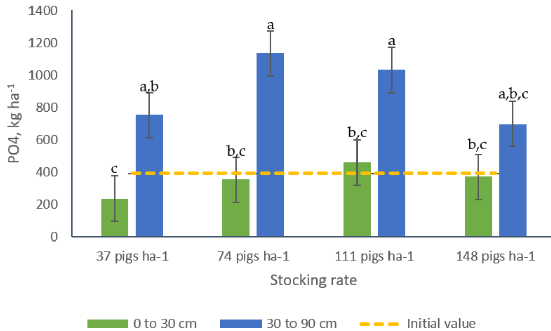
Figure 9. Effect of the interaction stocking rate \times sampling depth on soil PO 4 -P (kg ha -1 ) in bermudagrass paddocks grazed with pigs during two grazing periods. a, b, c: Means having the same letter are not significantly different at the 5% level of probability as indicated by the Multiple Comparisons test—simulate option. The Letter display does not reflect all significant comparisons. The following additional pairs are significantly different: SR148 SD30-90 vs. SR148 SD0-30; where SR: stocking rate and SD: sampling depth. Data are the means of three replicates. Errors bars represent plus or minus one standard error of the means within the interaction.
