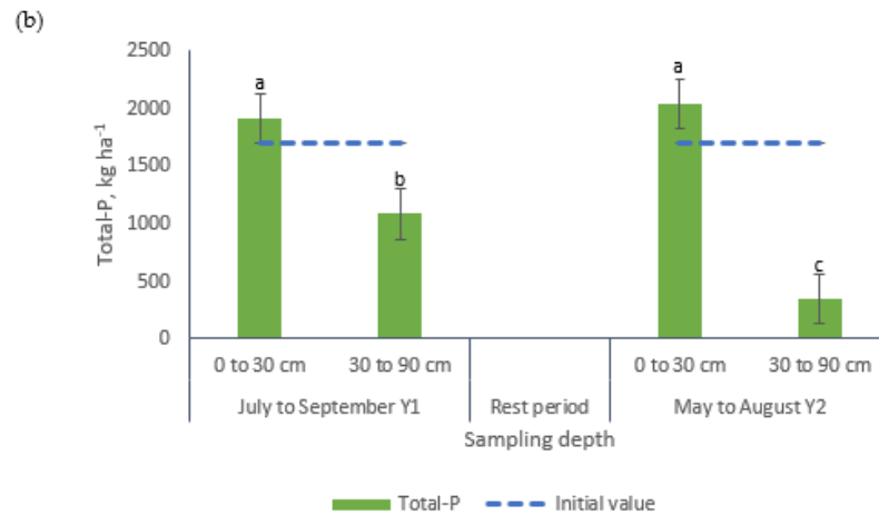
Figure 7. Effects of the interaction grazing period \times sampling depth on the concentrations ( \text{kg ha}^{-1} ) of (a) \text{PO}_4\text{-P} and (b) Total-P in soil samples from bermudagrass paddocks managed with different pig stocking rates for two 14-week grazing periods. a, b, c: Means having the same letter are not significantly different at the 5% level of probability as indicated by the Multiple Comparisons test—simulate option. Data are the means of three replicates. Errors bars represent plus or minus one standard error of the means within the interaction.
